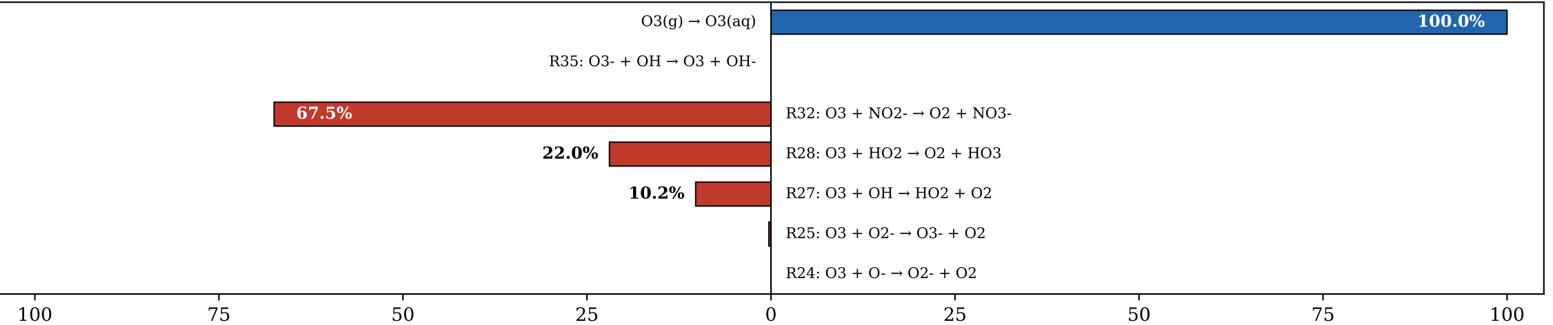
(c) \text{NO}_2^- ( \Sigma\text{src} = 6.01\text{e-}08 \text{ M/s} )
